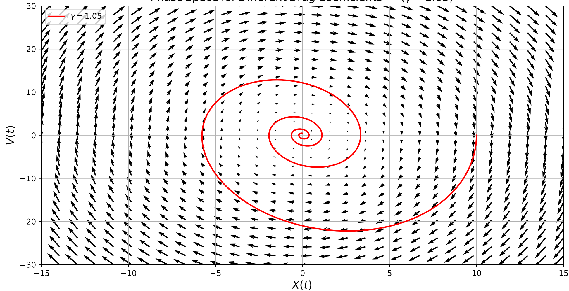
Phase Space for Different Drag Coefficients – ( \gamma = 1.05 )
